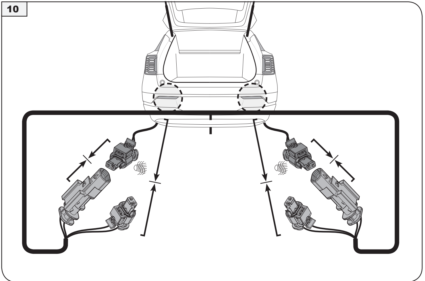
Modul Trail-tec 35-27 → Stecker 18 pin E-Satz modul Trail-tec 35-27 → socket 18 pin e-kit
